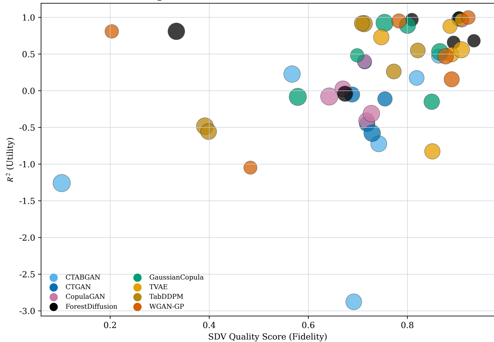
Regression bubble trade-off (size \propto MIA AUC)
